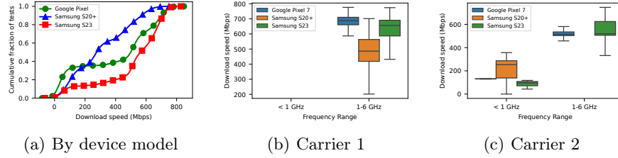
Fig. 7. Download speeds by frequency and device model (each with a different chipset).
