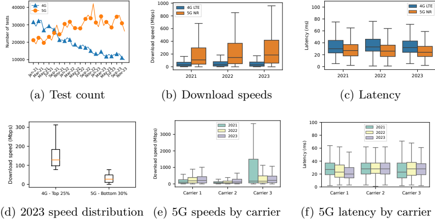
Fig. 1. Longitudinal evolution of test taking and measured download speeds.
