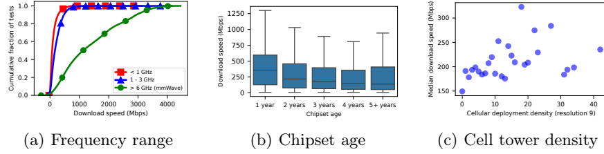
Fig. 2. Effect of key features in our dataset on measured downloads speeds.
