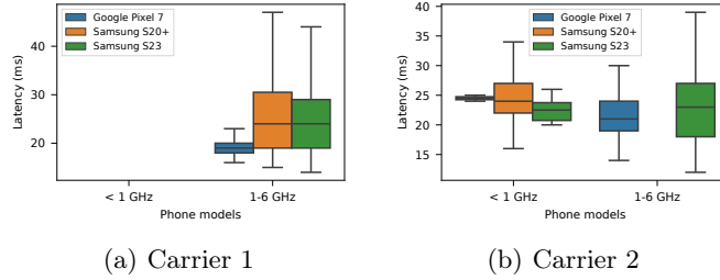
Fig. 8. Impact of frequency band and device chipset on latency.
