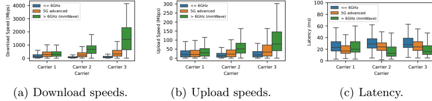
Fig. 3. Effect of frequency on measured network performance metrics.
