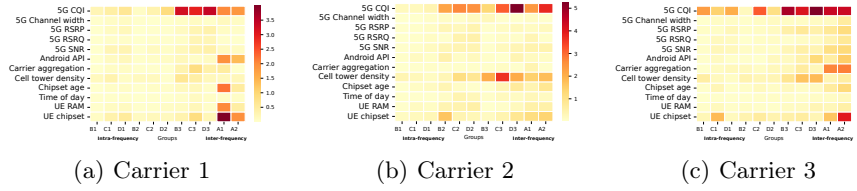
Fig. 5. KL divergence metrics - download speed.
