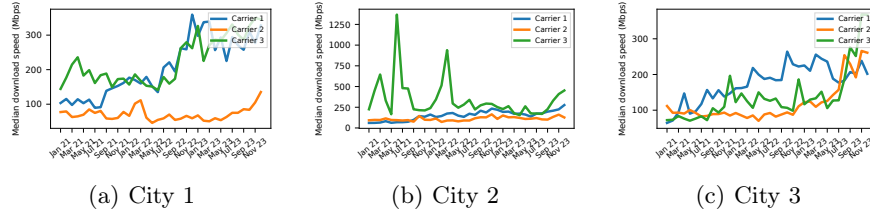
Fig. 9. Longitudinal performance of all three carriers in selected representative cities.
